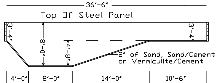
Finished Dim. for 17 x 37 Emerald
