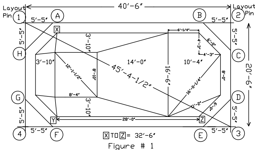
Excavation Layout Details for 17 x 37 Em.
